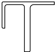
Bordure de finition US44 47.5 x 45.5 mm (1.9 x 1.8 po)
