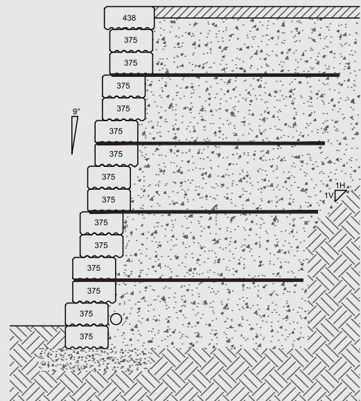
Grande Smooth Wall 3 m (9.8 ft.) 15 rows 9° reinforced slope
