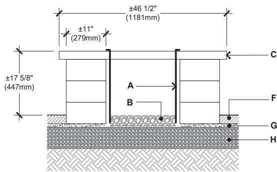
SECTION 1-1
