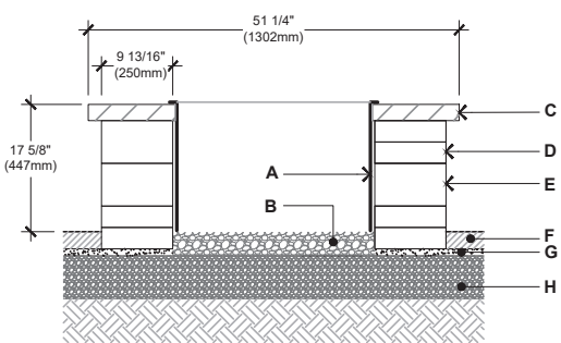
SECTION 1-1
