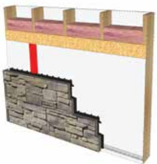
Standard framed wall with OSB or plywood and rigid insulation
